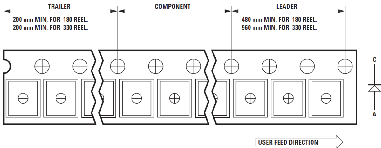
Figure 8. Tape Leader and Trailer Dimensions
