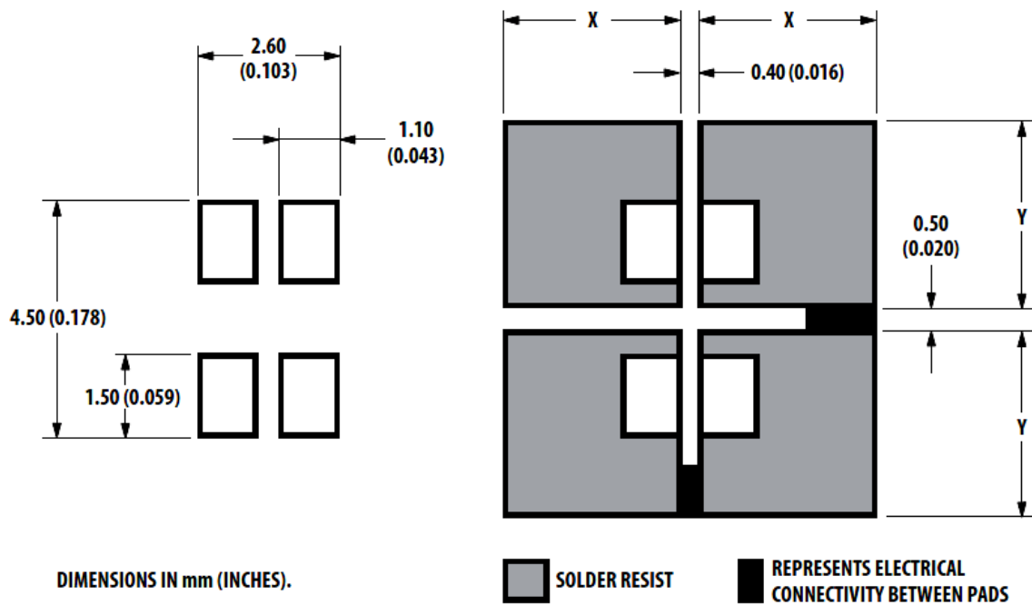
Figure 7. Recommended Soldering Pad Pattern
