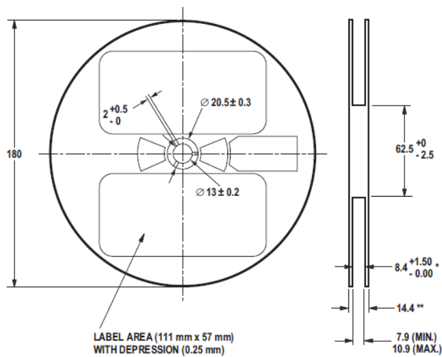
Figure 10. Reel dimensions
